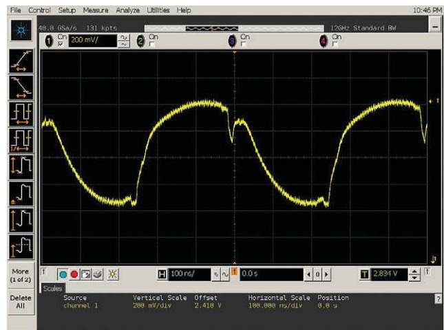
Figure 11. InfiniiScan's non-monotonic edge finder isolates a signal anomaly caused by a poor termination.
