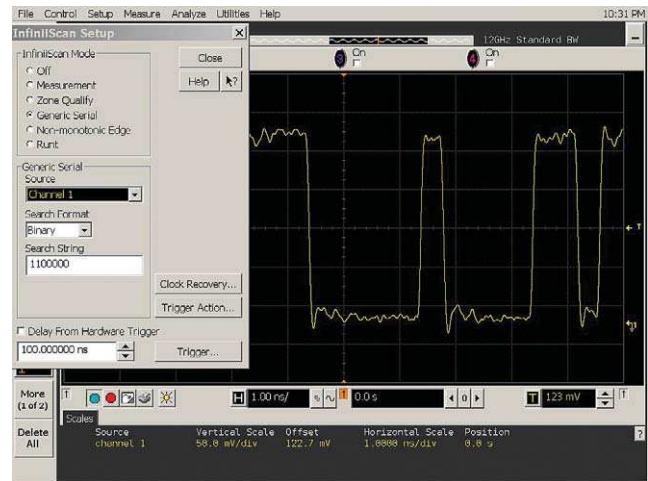
Figure 8. InfiniiScan’s generic serial finder is used to isolate a specific portion of a high-speed serial data stream.
