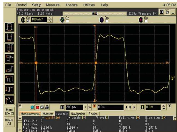
Figure 15. InfiniiScan measurement limit test simultaneously monitoring five different events (positive pulse width, negative pulse width, peak to peak voltage, fall time and rise time) on a single signal.
