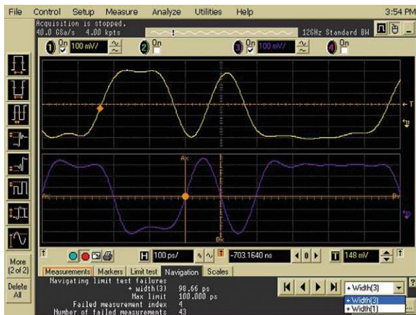
Figure 14. InfiniiScan measurement limit test identifying glitches on two channels simultaneously. Navigation controls (first, previous, next, last) also shown.
