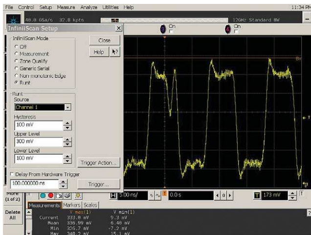
Figure 10. InfiniiScan's runt finder can be used to isolate runt pulses that occur in a signal.
