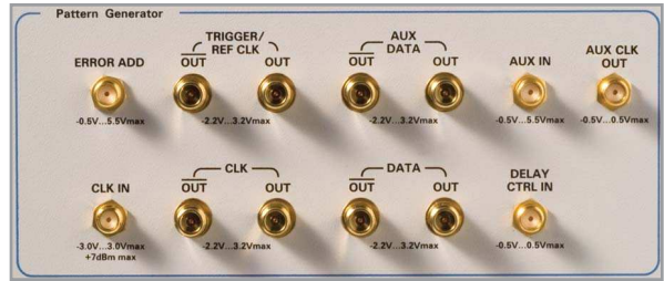
Figure 13. Generator connectors on front panel
