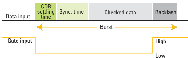
Figure 28. Burst mode allows recirculation loop testing
