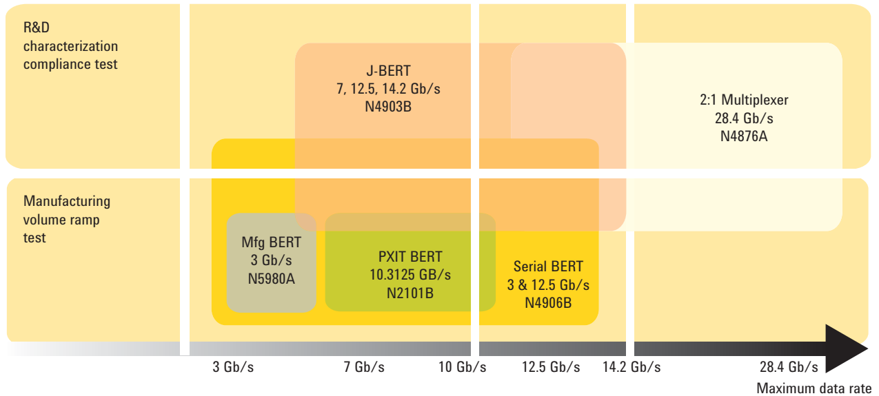
Figure 1. J-BERT is the highest-performance BERT amongst Agilent's offering of serial BERT solutions for R&D and manufacturing
