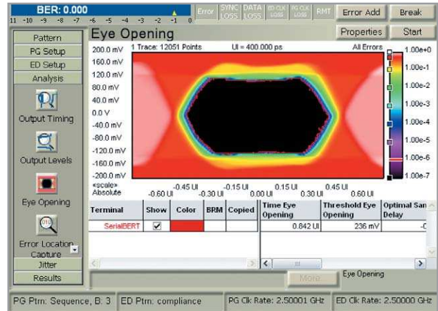
Figure 8. Eye contour with colors indicating BER level
