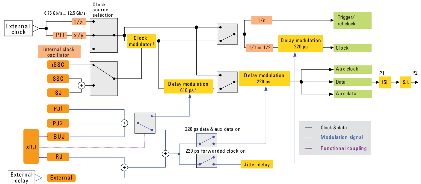
Figure 22. Overview of jitter injection capabilities
