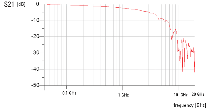
Figure 24. Typical S21 parameter for ISI channel of 9 inch length
