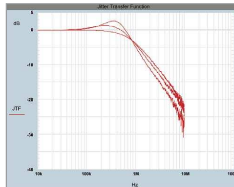
Figure 27. Three selectable frequency response settings. The example shows JTF loop bandwidth of 900 kHz and 0 dB, 1.2 dB, 2.8 dB peaking
