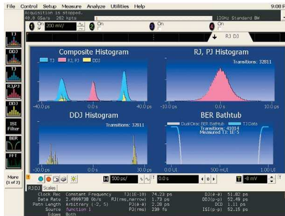
Figure 6. Total jitter analysis by Rj/Dj decomposition through N5400A EZJIT Plus jitter analysis software
