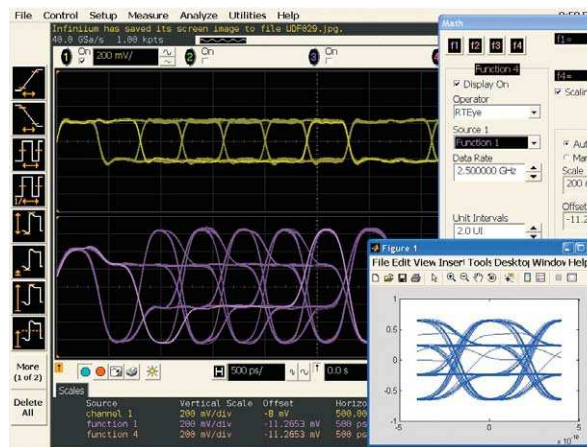
Figure 5. The eye pattern of an equalized signal created using E2688A high-speed serial data analysis software and the MATLAB plotting feature.
