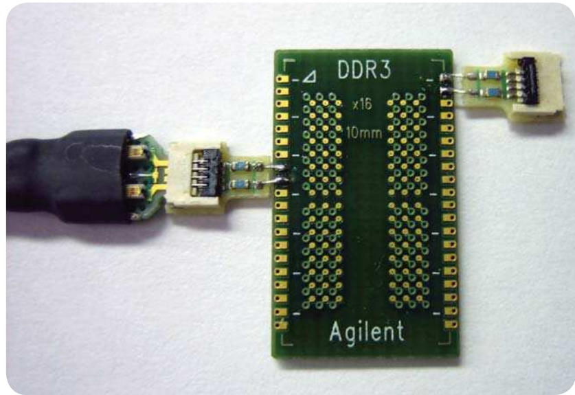
Figure 2. The picture above shows the InfiniiMax N5425A and N5426A ZIF probe head connected to the W2636A DDR3 BGA probe adapter.
