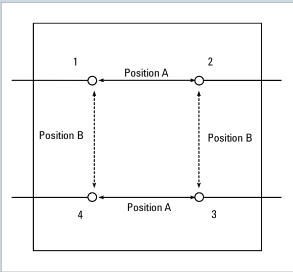
M9156C is an integration of 2 units of Agilent L7222C with Option 161 (24 V, 10-pin DIP)
