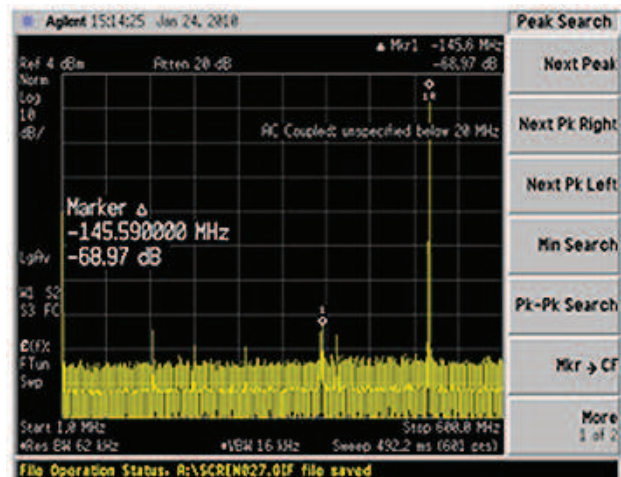
Figure 4. Spurious performance of 81180A
