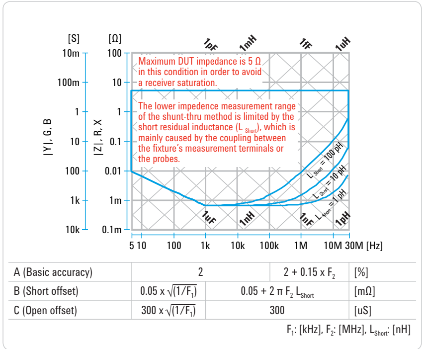
Figure 7. Impedance measurement accuracy (SPD) \leq 10\% , Gain-phase shunt-thru method (T: 50 Ω 0 dB, R: 50 Ω 20 dB).
