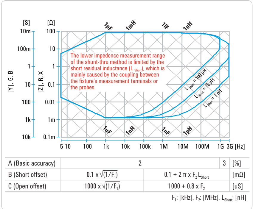
Figure 6. Impedance measurement accuracy (SPD) \leq 10\% , S-parameter port 1-2 shunt-thru method.
