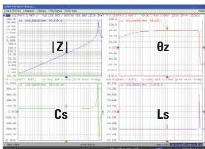
RF inductor measurement with reflection method (1 MHz to 3 GHz)
