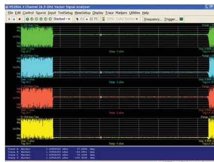
Multi channel phase coherent Vector Signal Analysis
