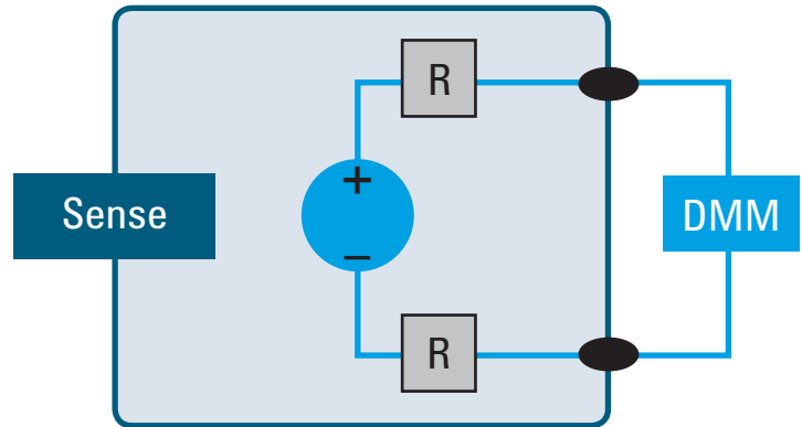
Figure 1. Basic example of the SENSE mechanism
