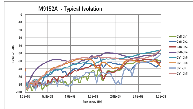
M9152A Typical Isolation
