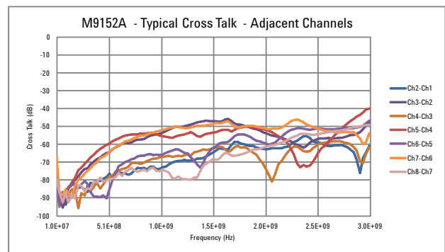
M9152A Typical cross talk-adjacent channels
