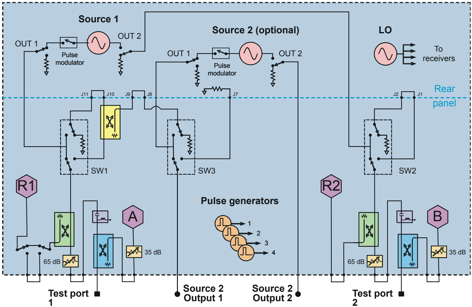
Figure 21. 2-Port N5241A and N5242A (Option 219, 224), Showing J-Designators for Rear Panel Connectors
