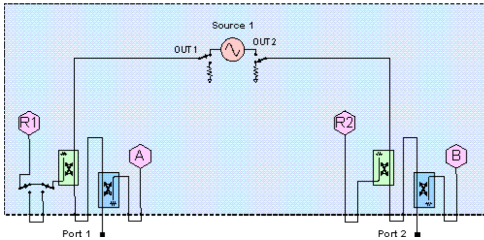
Figure 16. 2-Port N5241A and N5242A (Option 219)
