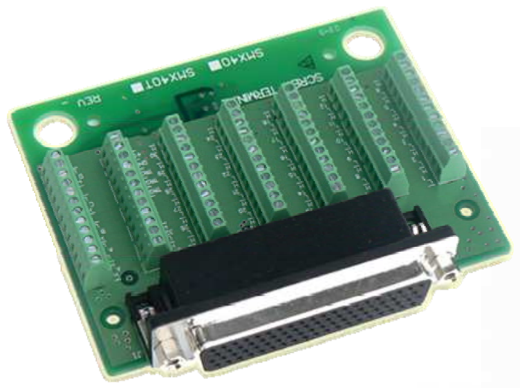
The SMX40 provides a convenient way to make Connections to the 4030 and 4032 models.
