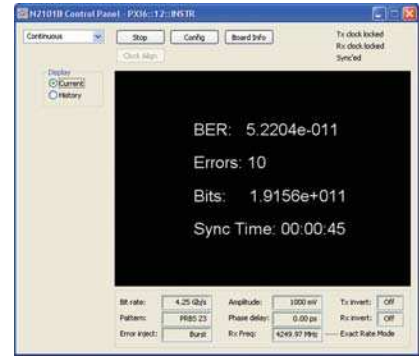
Bit Error Rate: Continuous Mode
