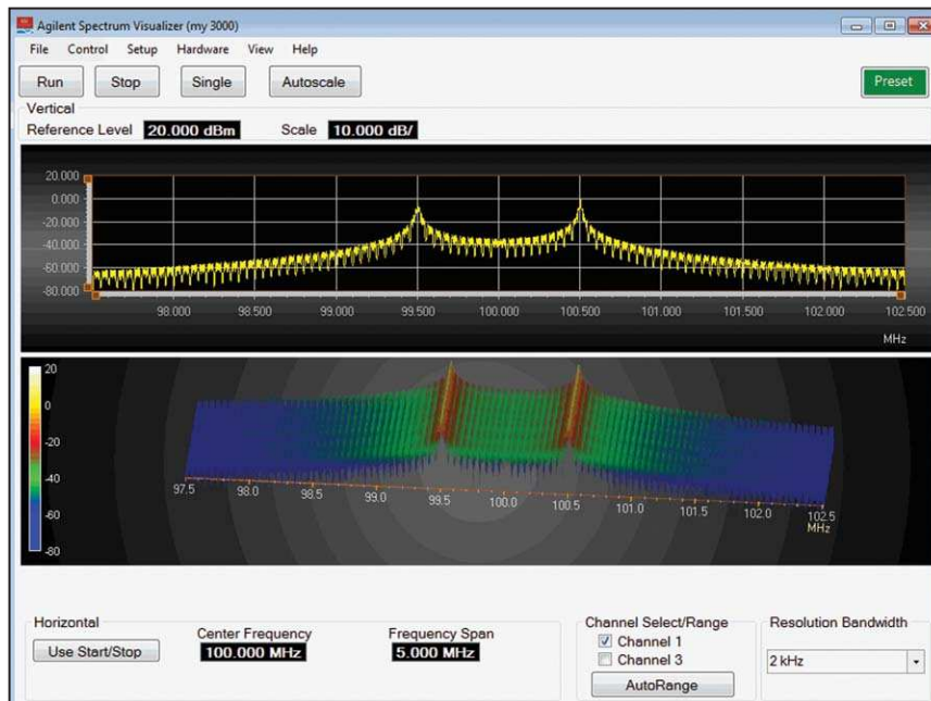
Figure 2: Waterfall view for ASV spectrogram measurement
