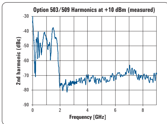
Harmonics (measured)
