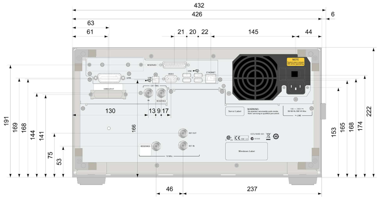
Figure 13. Rear view
