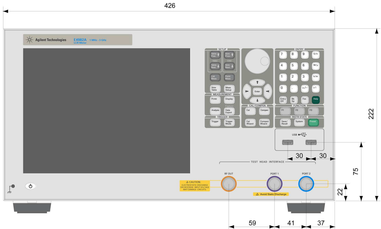
Figure 12. Front view
