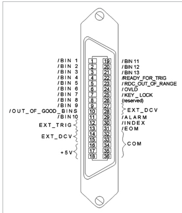
Figure 11. Pin assignment
