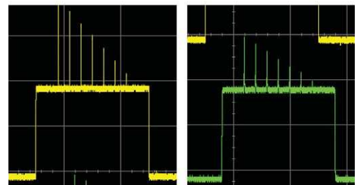
Trueform at 50 kHz DDS at 50 kHz
