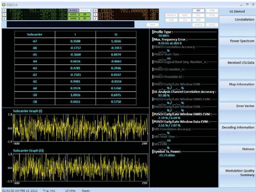
Figure 4. N6061A IQ data measurement
