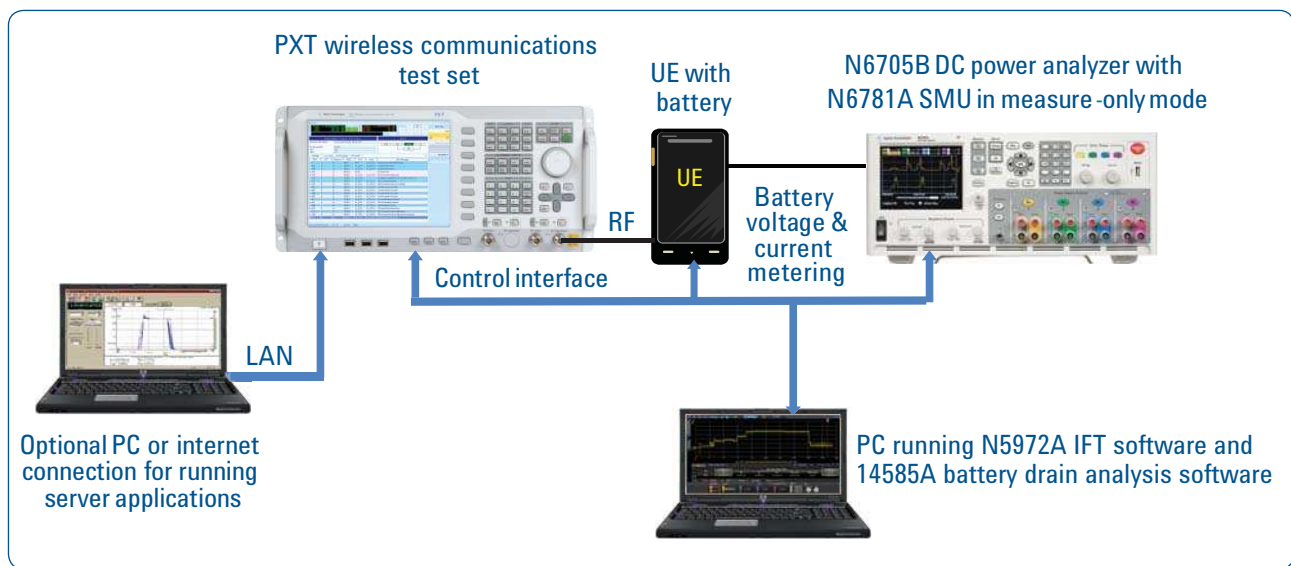
Figure 7. Interactive functional test system
