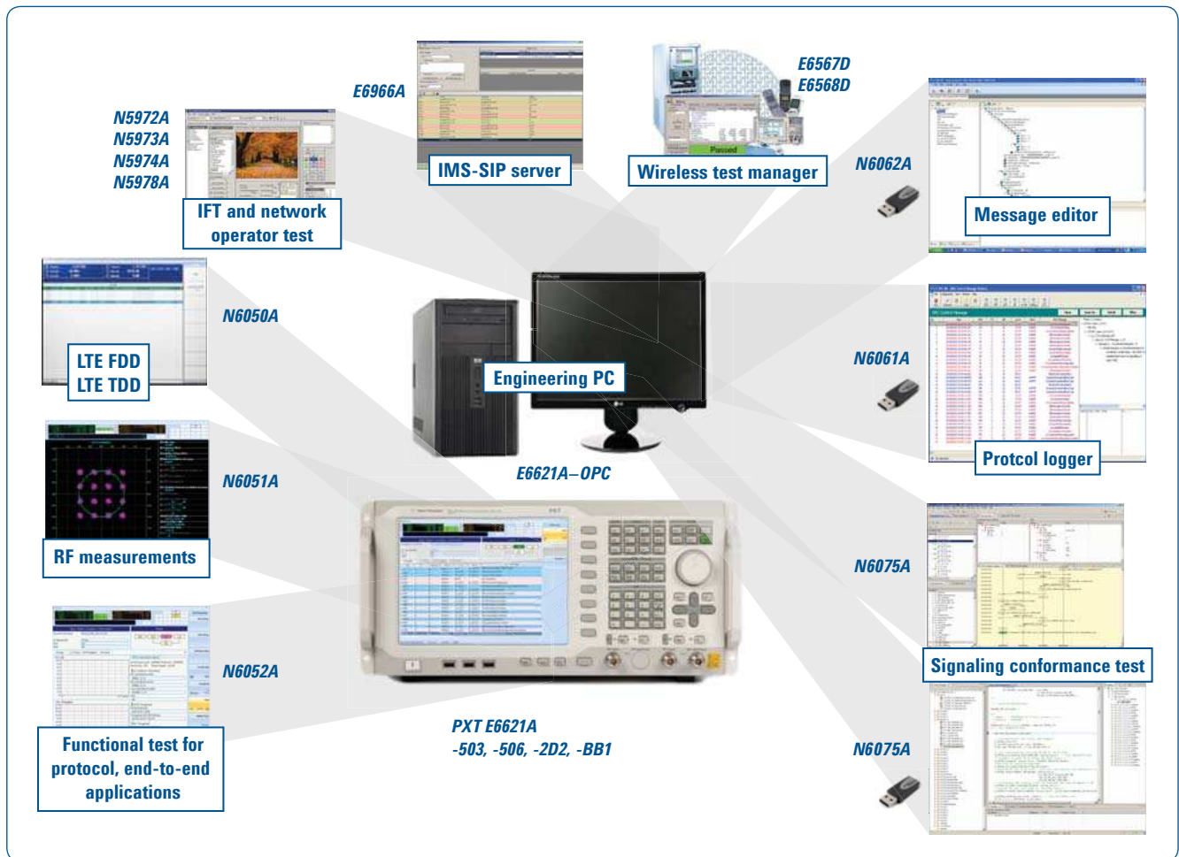
Figure 10. Maximum flexibility to satisfy all configuration needs
