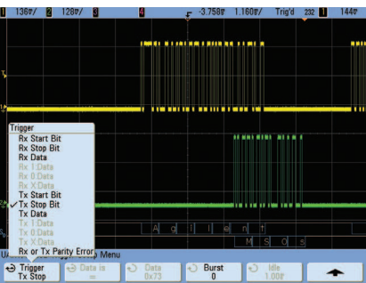
Trigger on and decode RS-232/UART transmission.
