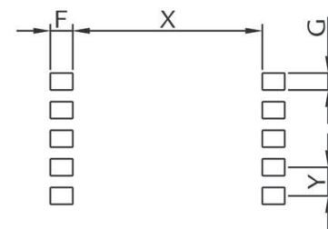
Top View Recommended PCB Layout
