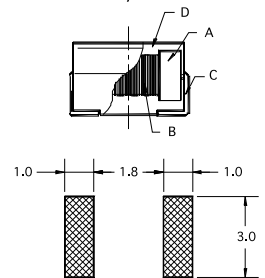
Pad layout
