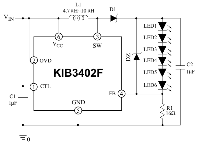
Figure5. 6LEDs driver with Open-circuit protection.
