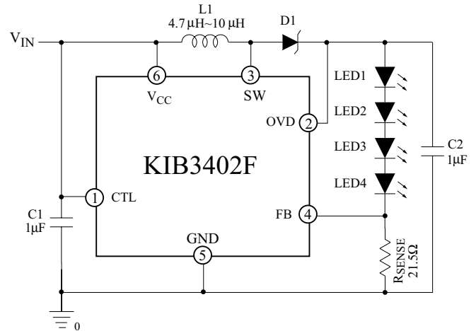
Figure4. 4LEDs driver with Open-circuit protection.
