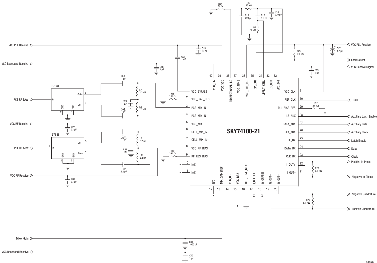
Figure 3. SKY74100-21 Application Schematic
