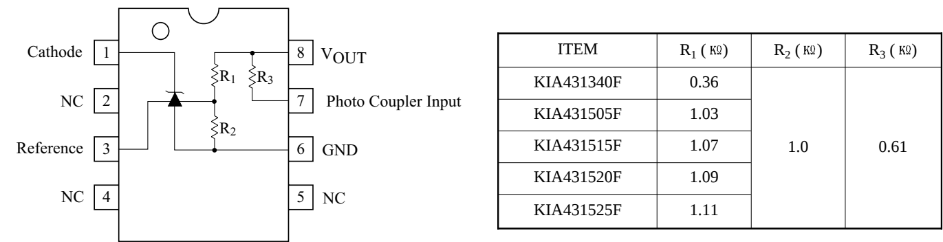
Fig. 1 BLOCK DIAGRAM
