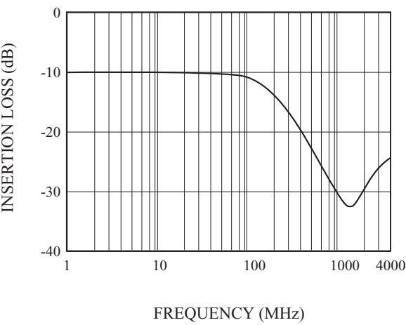
S_{21} - f
