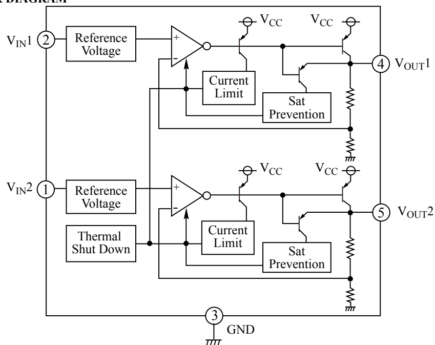
BLOCK DIAGRAM
