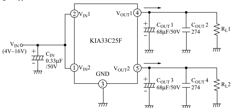
Fig.2 Application Circuit
