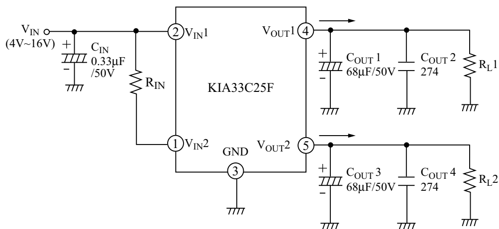
Fig.2 Application Circuit
