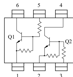
EQUIVALENT CIRCUIT (TOP VIEW)
