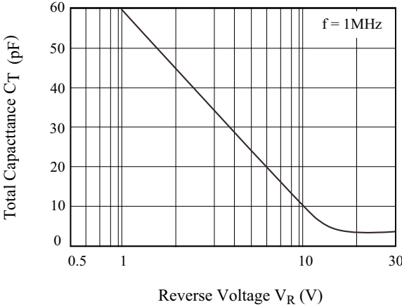
C_R - V_R
