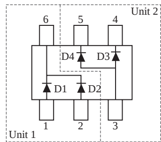
EQUIVALENT CIRCUIT (TOP VIEW)
