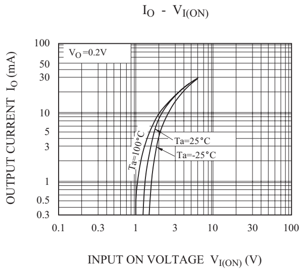
Q 2 (NPN TRANSISTOR With Built-in Bias Resistors)
