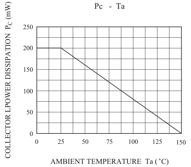
TOTAL POWER DISSIPATION
