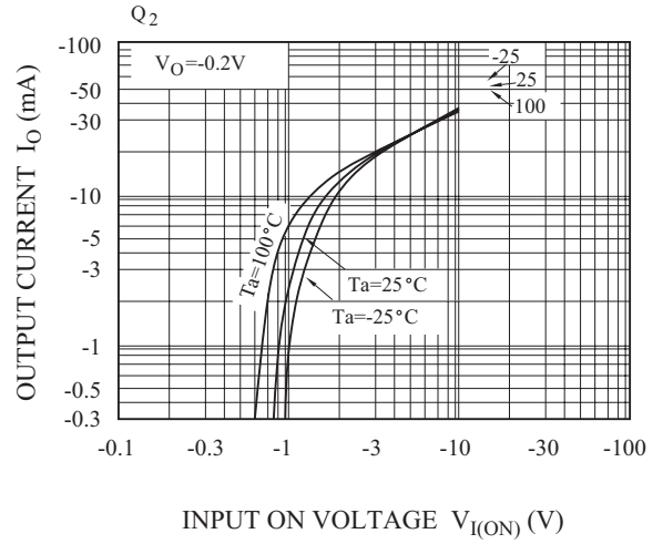
I_O - V_{I(ON)}
