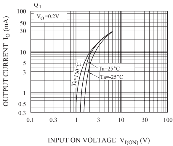
I_O - V_{I(ON)}
