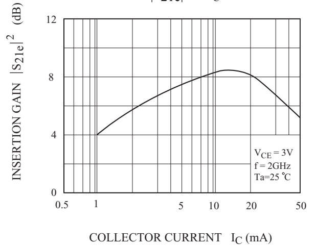
|S_{21e}|^2 - I_C
