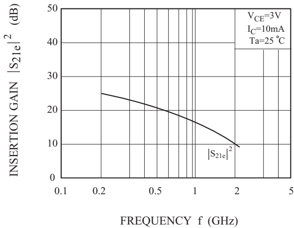
|S_{21e}|^2 - f
