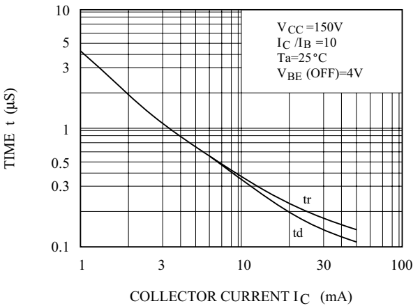
TURN-ON SWITCHING CHARACTERISTICS
