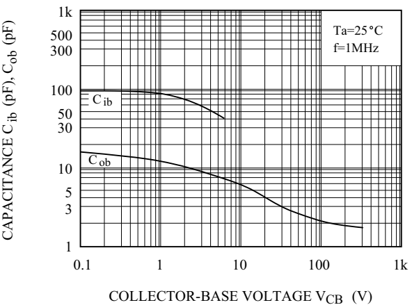
C_{ib}, C_{ob} - V_{CB}
