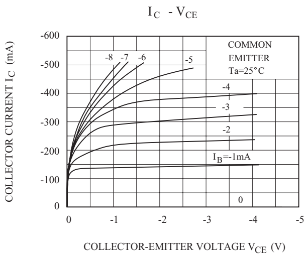
Q 2 (PNP TRANSISOR)
