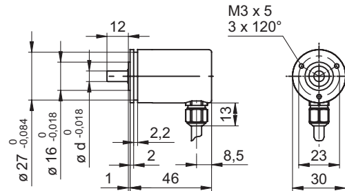
BMSV/BMMV 30R CANOpen, cable radial
