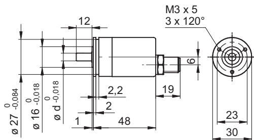
BMSV/BMMV 30R CANOpen, connector axial
