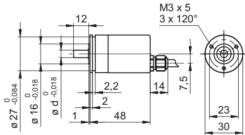
BMSV/BMMV 30R CANOpen, cable axial
