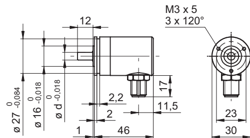
BMSV/BMMV 30R CANOpen, connector radial
