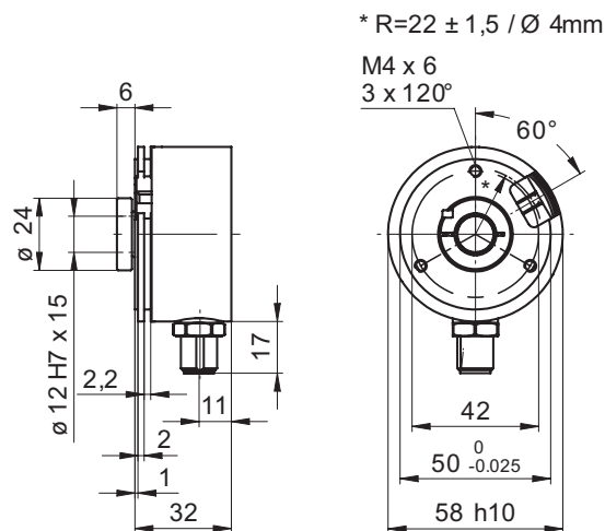
BMSH/BMMH 58 CANopen connector 1 x M12 radial
