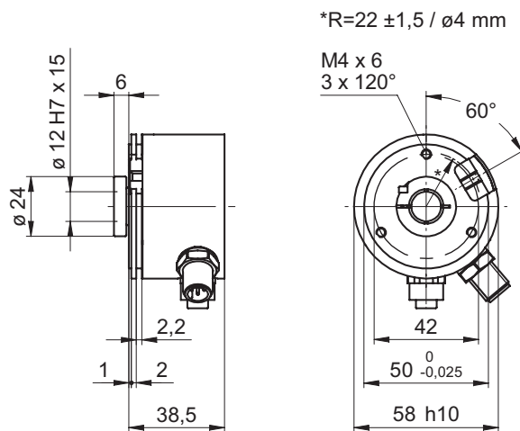
BMSH/BMMH 58 CANopen connector 2 x M12 radial
