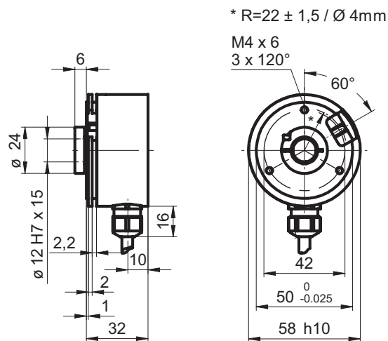
BMSH/BMMH 58 CANopen cable radial
