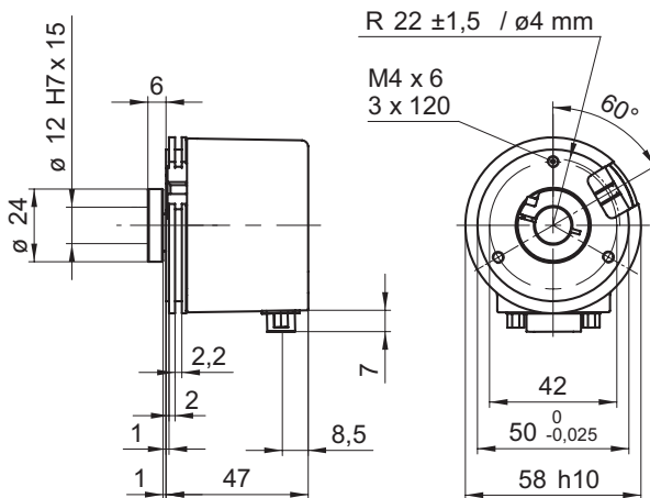
BMSH/BMMH 58 CANopen connector D-SUB radial
