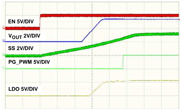
FIGURE 21. SOFT-START AT NO LOAD, 500 \mu s/DIV
