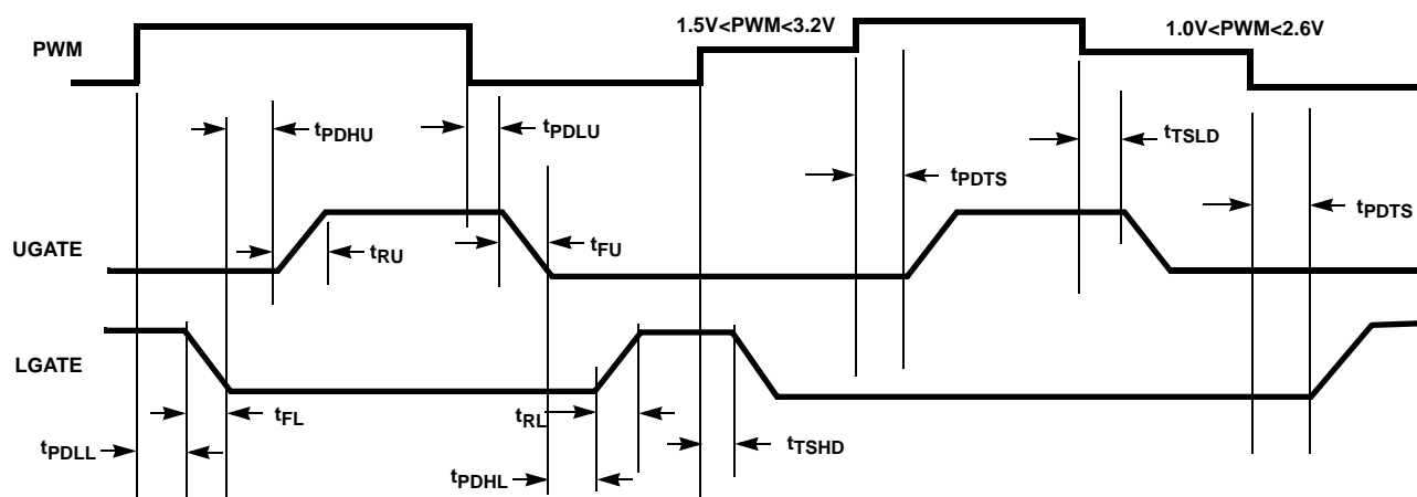
FIGURE 1. TIMING DIAGRAM
