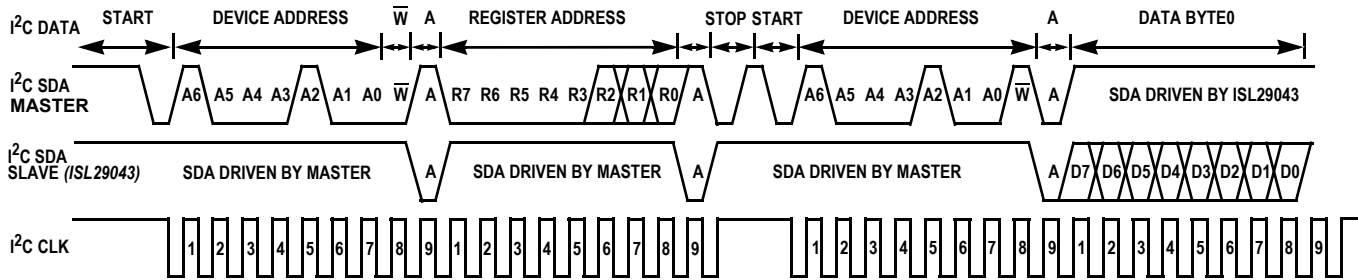
FIGURE 4. I²C DRIVER TIMING DIAGRAM FOR MASTER AND SLAVE CONNECTED TO COMMON BUS
