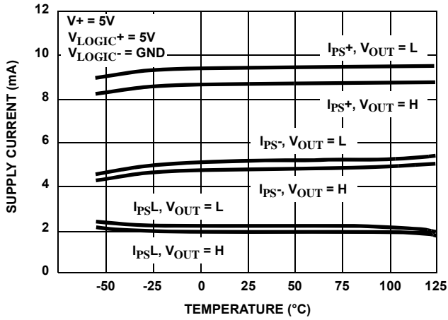
FIGURE 4. SUPPLY CURRENT vs TEMPERATURE (FOR ±15V SUPPLIES AND +5V LOGIC SUPPLY)
