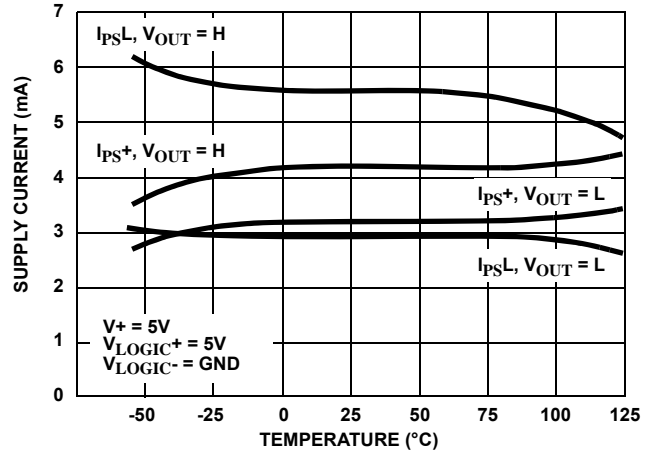
FIGURE 5. SUPPLY CURRENT vs TEMPERATURE (FOR SINGLE +5V OPERATION)
