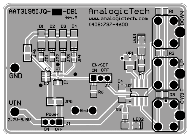
Figure 4: AAT3195 Evaluation Board Top Side Layout.
