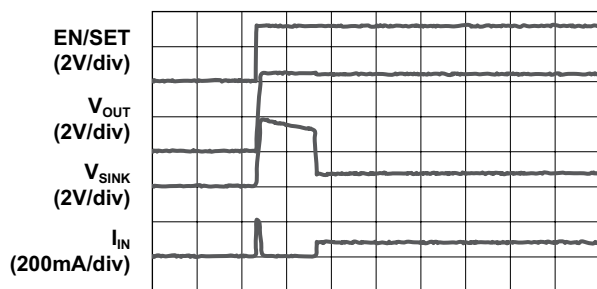
Turn On to 1X Mode ( V_{IN} = 4.2V ; 20.5mA/ch)
