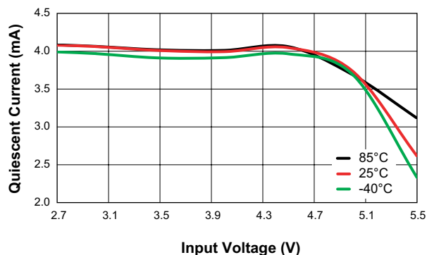
No Load Operating Current vs. Input Voltage
