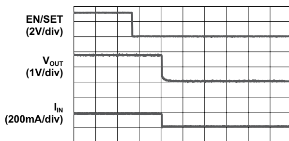
Turn Off from 2X Mode (20.5mA/ch)
