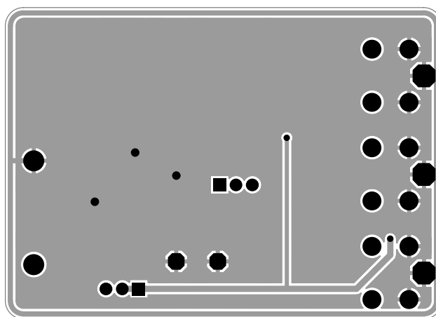
Figure 5: AAT3195 Evaluation Board Bottom Side Layout.
