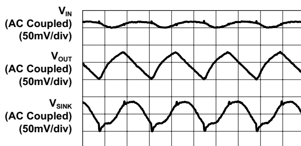
AAT3195-2 Output Ripple Waveform ( V_{IN} = 3.6V ; 2X Mode; 20.5mA Load)
