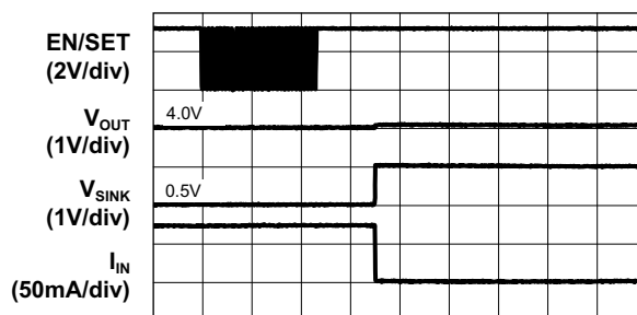
Transition of LED Current (20.5mA to 1.3mA)
