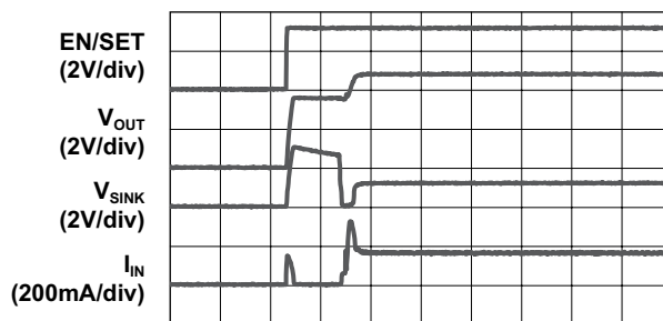
Turn On to 2X Mode ( V_{IN} = 3.6V ; 20.5mA/ch)
