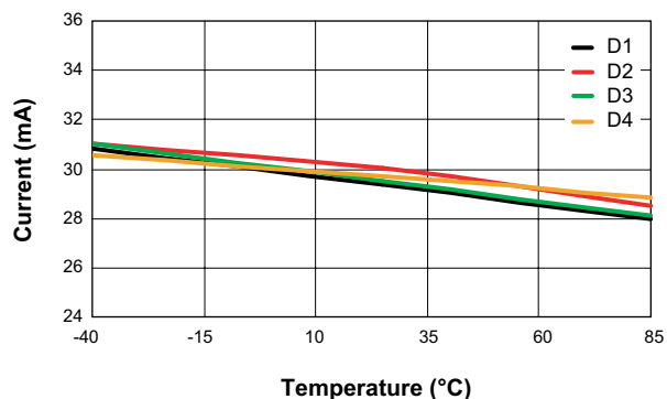
AAT3195-1 Current Matching vs. Temperature ( V_{IN} = 3.6V )
