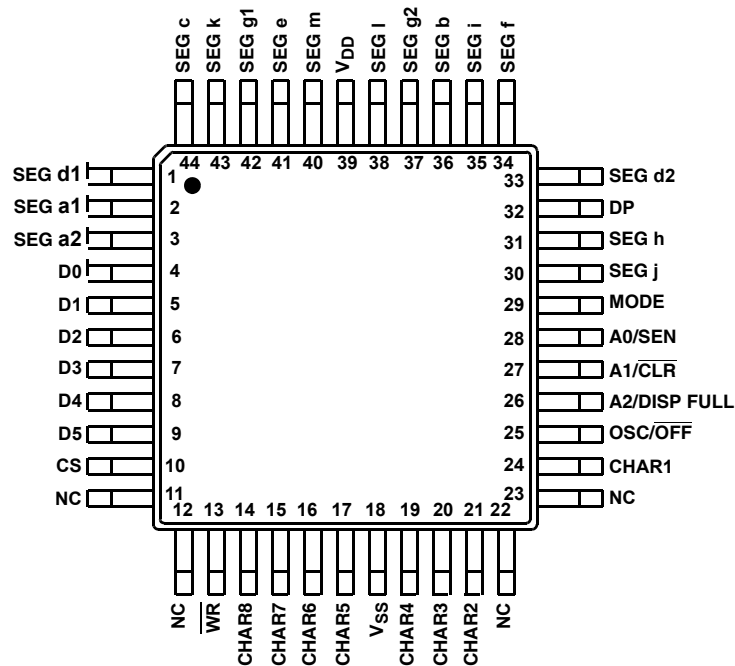
ICM7243A (16-SEGMENT CHARACTER) (44 Ld MQFP) TOP VIEW
