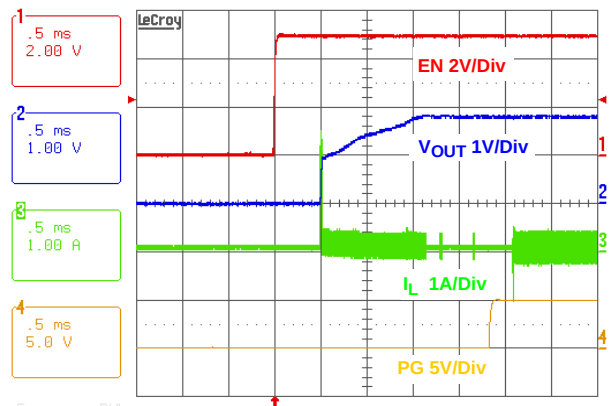
FIGURE 36. SOFT-START WITH NO LOAD (PWM)
