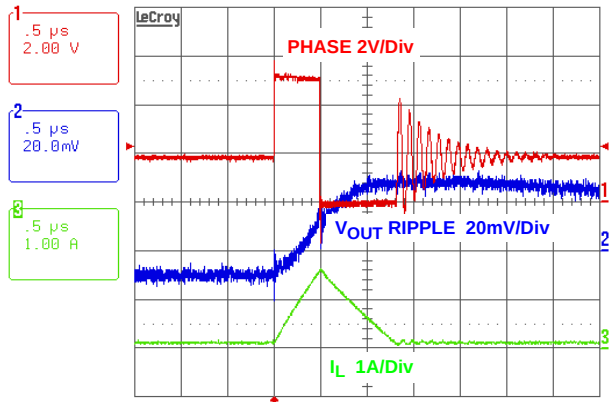
FIGURE 34. STEADY STATE OPERATION AT NO LOAD (PFM)
