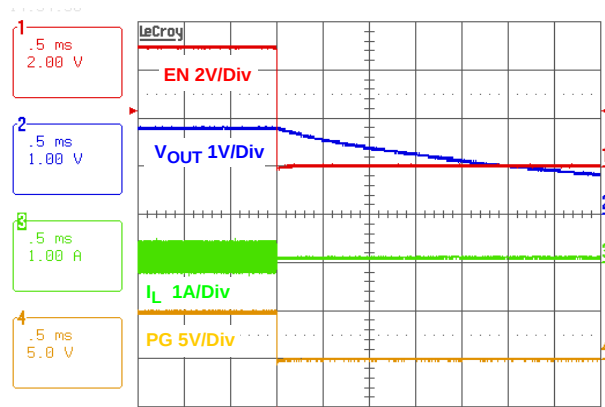
FIGURE 39. SOFT-DISCHARGE SHUTDOWN
