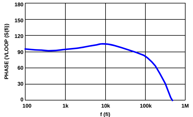
FIGURE 44. SIMULATED LOOP GAIN
