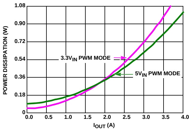
FIGURE 9. POWER DISSIPATION vs LOAD (1MHz, V_{OUT} = 1.8\text{V} )
