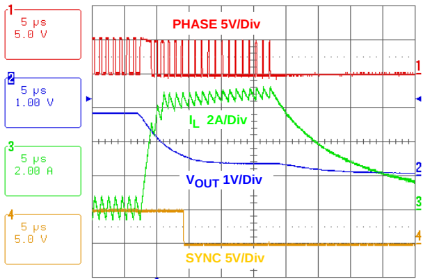
FIGURE 31. OUTPUT SHORT CIRCUIT
