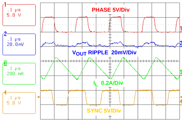
FIGURE 29. STEADY STATE OPERATION AT NO LOAD WITH FREQUENCY = 4MHz
