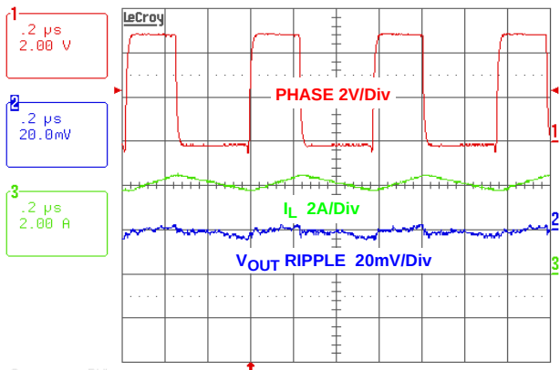
FIGURE 35. STEADY STATE OPERATION WITH FULL LOAD
