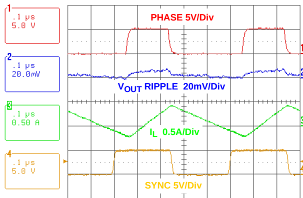
FIGURE 27. STEADY STATE OPERATION AT NO LOAD WITH FREQUENCY = 2MHz
