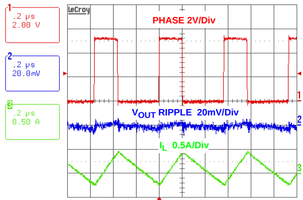
FIGURE 33. STEADY STATE OPERATION AT NO LOAD (PWM)
