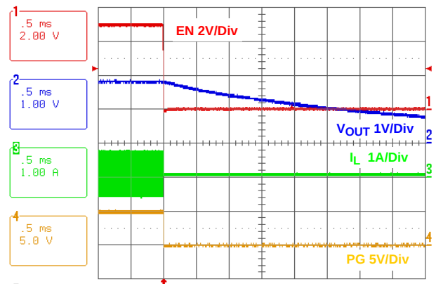
FIGURE 26. SOFT-DISCHARGE SHUTDOWN
