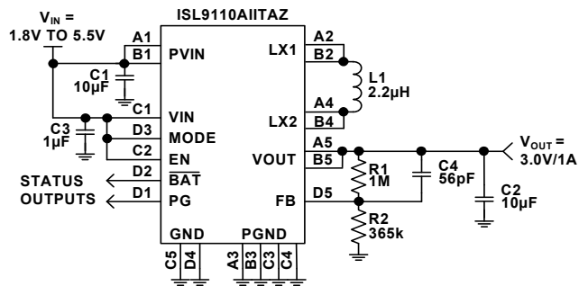
FIGURE 28. TYPICAL ISL9110AIIAZ APPLICATION
