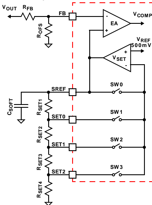
FIGURE 7. VOLTAGE PROGRAMMING CIRCUIT
