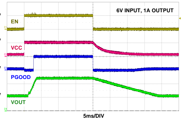
FIGURE 11. ENABLE/DISABLE WAVEFORMS
