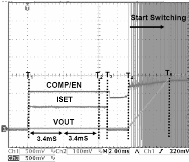
FIGURE 15. I_{SET} AND SOFT-START OPERATION
