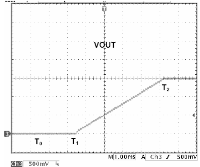
FIGURE 16. NORMAL START-UP
