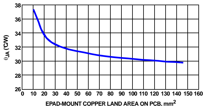
FIGURE 12. θ JA vs EPAD-MOUNT COPPER LAND AREA ON PCB
