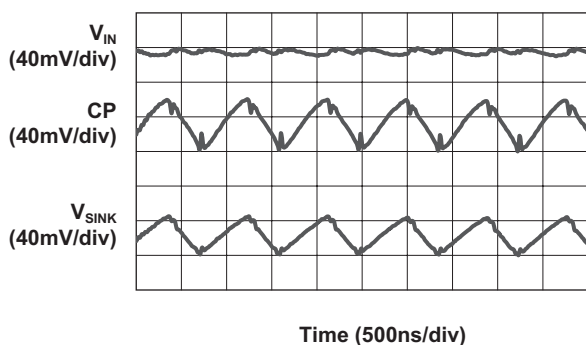
Load Characteristics ( V_{IN} = 4.0V ; 1.5X Mode; 20mA/Channel)
