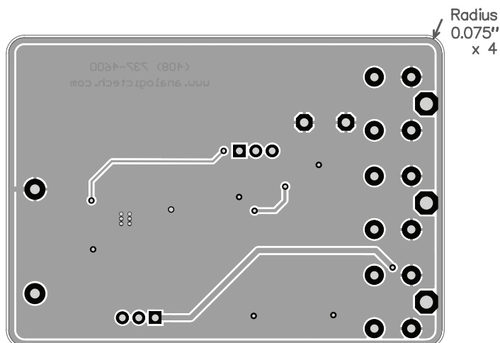
Figure 7: AAT3169ISN Evaluation Board Bottom Side Layout.
