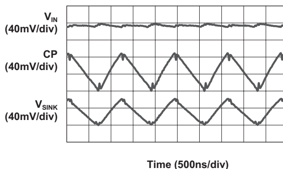
Load Characteristics ( V_{IN} = 2.9V ; 2X Mode; 15mA/Channel)
