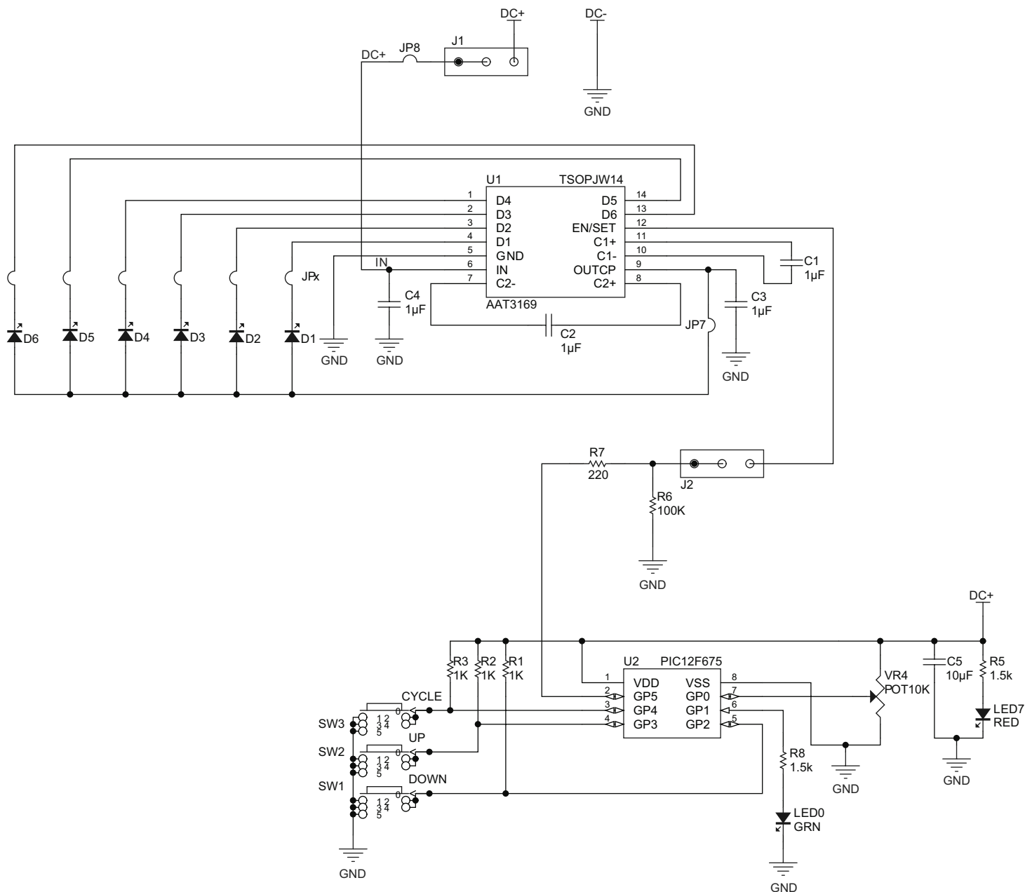
Figure 3: AAT3169ITO Evaluation Board Schematic.
