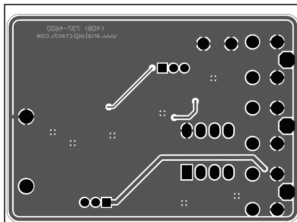
Figure 9: AAT3169ITO Evaluation Board Bottom Side Layout.
