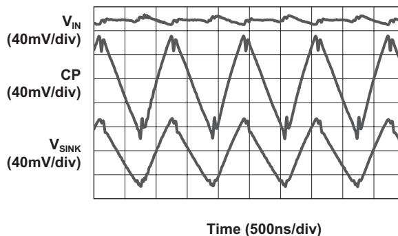
Load Characteristics ( V_{IN} = 3.6V ; 2X Mode; 30mA/Channel)
