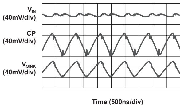
Load Characteristics ( V_{IN} = 4.3V ; 1.5X Mode; 30mA/Channel)
