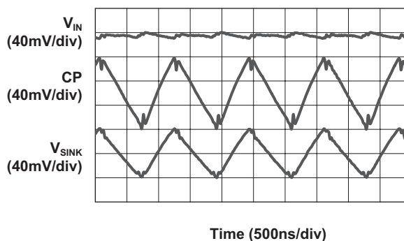
Load Characteristics ( V_{IN} = 3.1V ; 2X Mode; 20mA/Channel)
