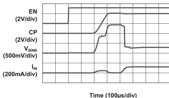
Turn-On to 1X Mode ( V_{IN} = 4.2V ; 20mA/Channel)
