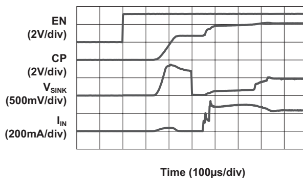
Turn-On to 2X Mode ( V_{IN} = 2.8V ; 20mA/Channel)
