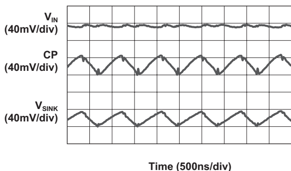
Load Characteristics ( V_{IN} = 3.8V ; 1.5X Mode; 15mA/Channel)
