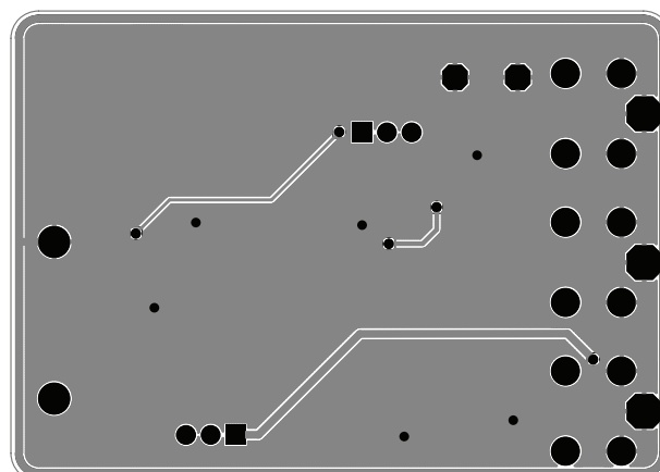
Figure 5: AAT3169IFO Evaluation Board Bottom Side Layout.
